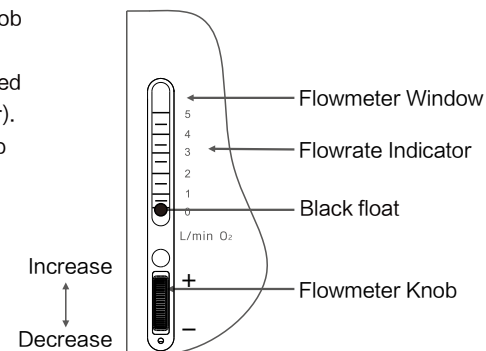
Figure 7: Setting Flowrate
