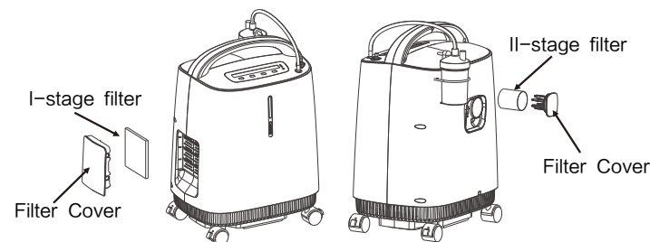
Figure 9: Remove Filter
