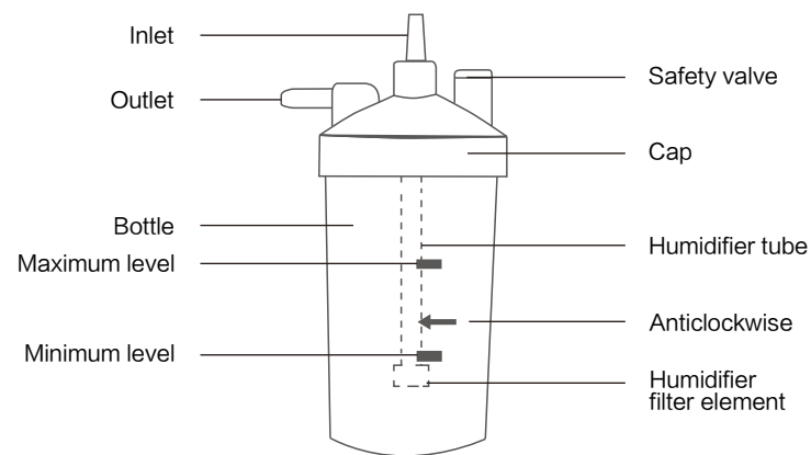
Figure 5: Humidifier Components
